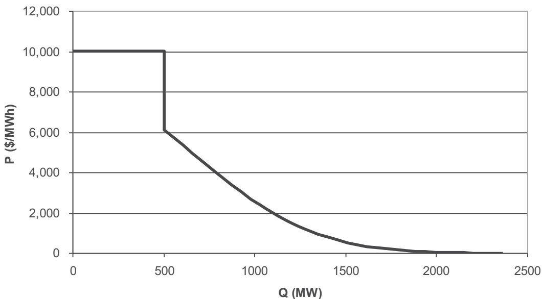
FIGURE 1 Operating Reserve Demand
